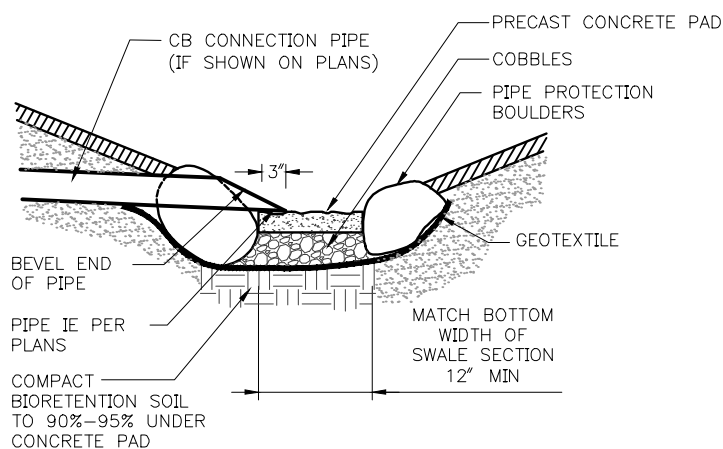
SECTION A-A (ENLARGEMENT)
