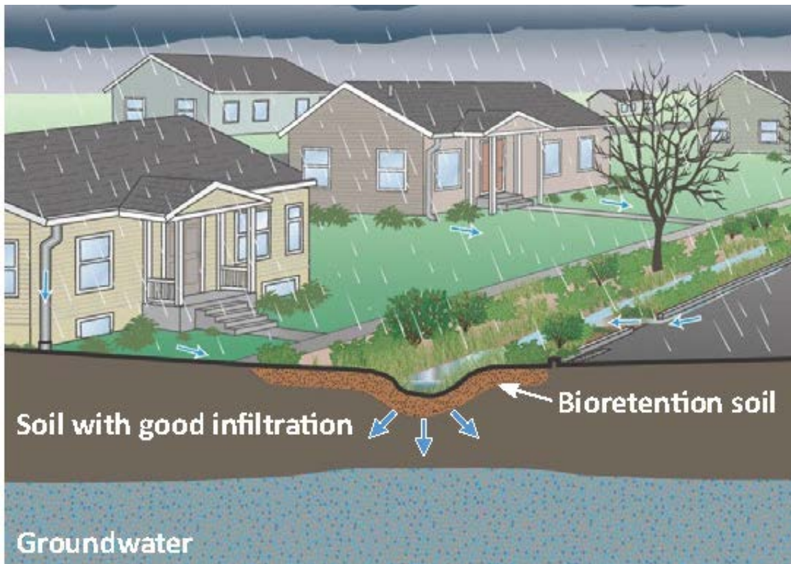
Image Bioretention with shallow infiltration (no underdrain) in planting strip. Graphic from WTD Barton project outreach materials.
