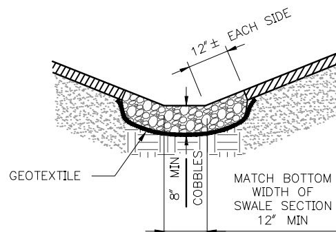
SECTION B-B (ENLARGEMENT)
