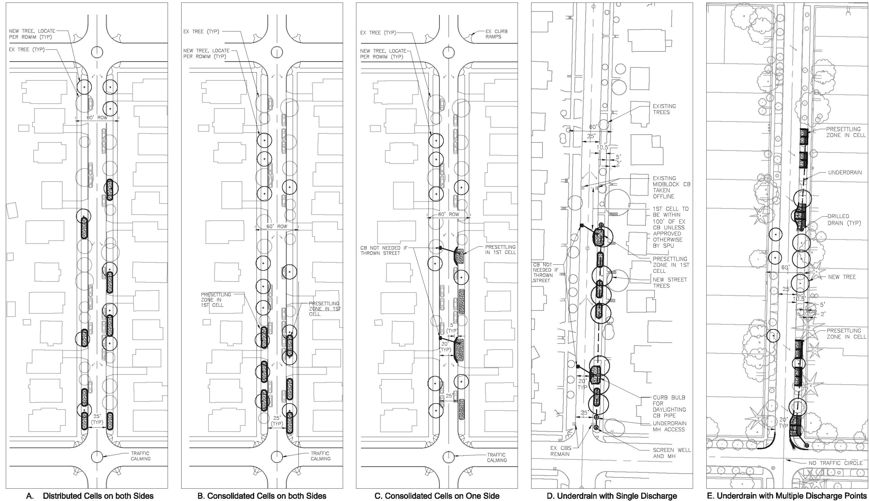
Figure 7-1: Block concepts for managing flow from a single Neighborhood Yield Street for varying site conditions and design approaches
