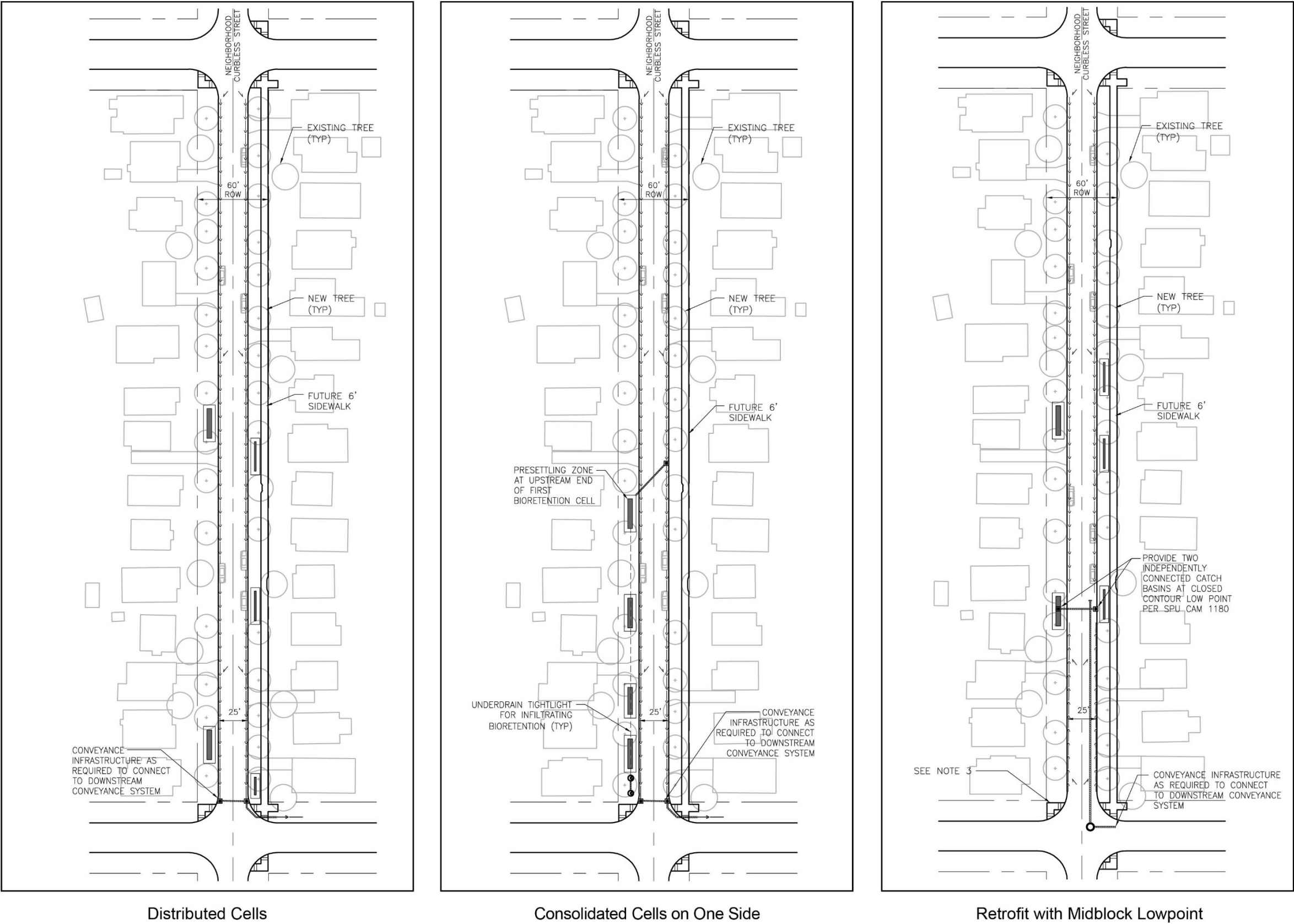
Figure 7-2: Block concepts for managing flow from a Neighborhood Curbless street
