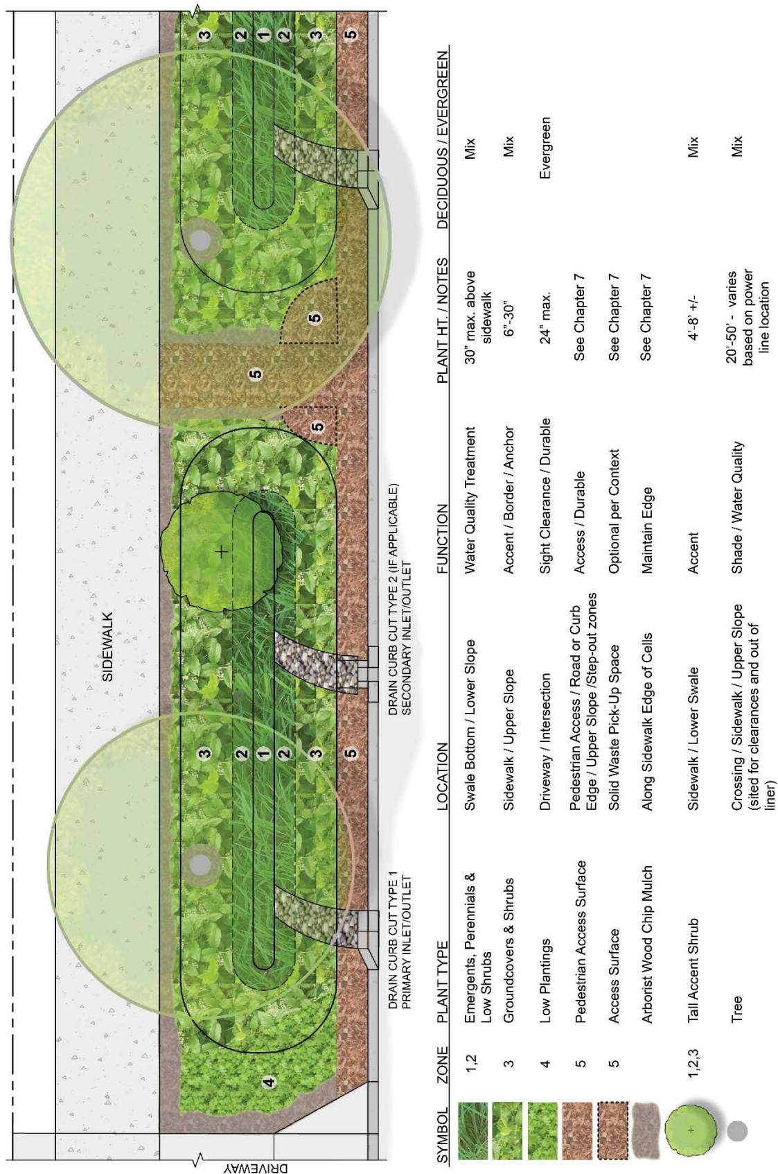
Figure 7-31: ROW bioretention cell planting zone diagram
