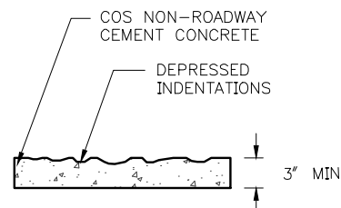
PRECAST CONCRETE PAD SECTION
