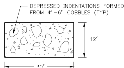
PRECAST CONCRETE PAD PLAN
