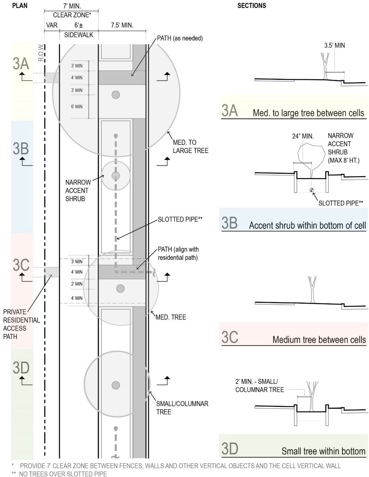
Figure 8-2: Tree placement at bioretention cell with 4 vertical walls -Placeholder
