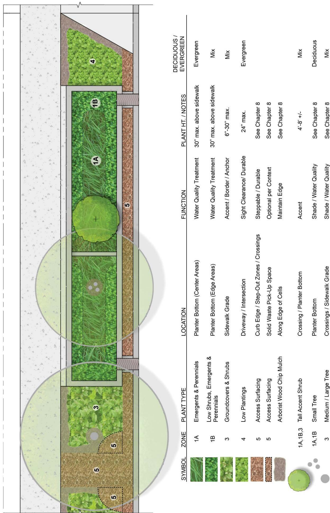
Figure 8-1: ROW bioretention planter planting zone - placeholder
