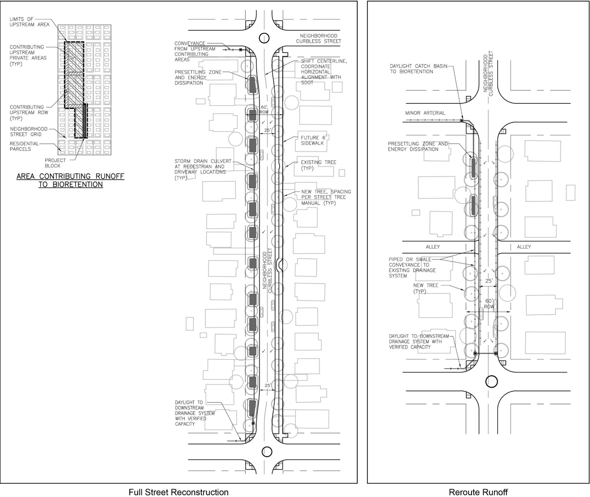
Figure 7-3: Distributed cells block concepts, retrofit to manage flow from upstream blocks onto a Neighborhood Curbless street
