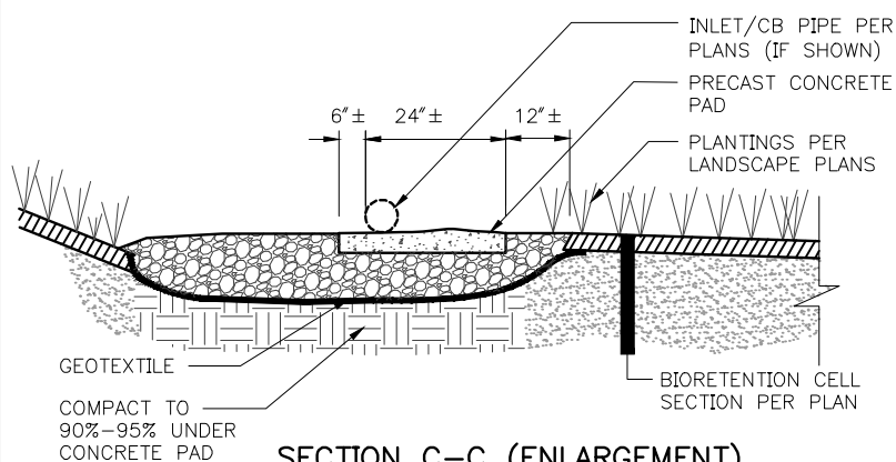
SECTION C-C (ENLARGEMENT)
